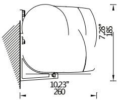
Wall installation
