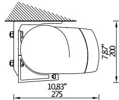
Ceiling installation
